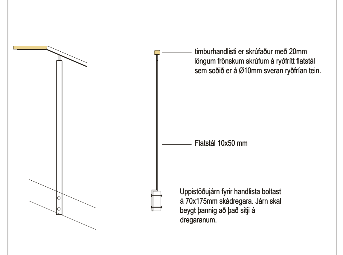
Handlisti, festing - Mkv. 1:20
